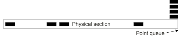
Figure 10.5: Envisioning a point queue as vehicles stacking vertically.
