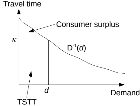
Figure 9.1: Relationship between inverse demand function, consumer surplus, and total system travel time.
