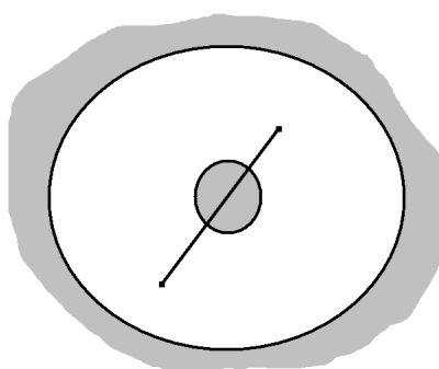
Figure 3.4: A nonconvex set with a “hole” in it.
