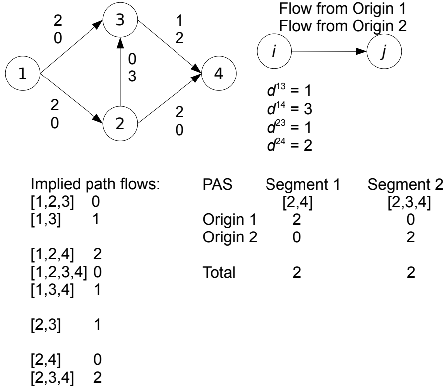
Figure 7.26: Example of a proportionality adjustment for a non-isolated PAS.
