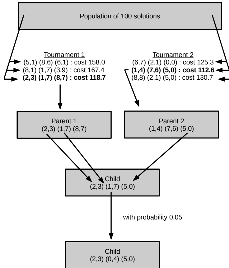
Figure 3.15: Generation of a new solution: reproduction and mutation.
