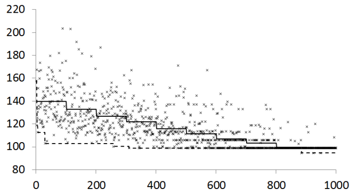
Figure 3.16: Progress of genetic algorithm. Solid line shows average generation cost, dashed line best cost so far, crosses cost of individual solutions.
