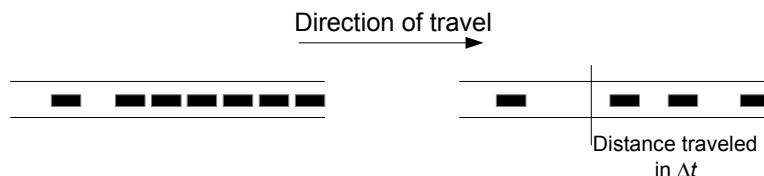
Figure 9.2: Calculating the sending flow when there is a queue on the link (left) and when the link is at free-flow (right).
