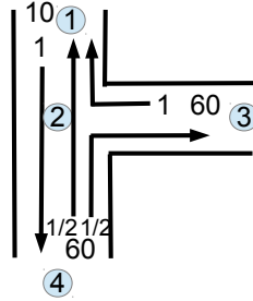
Figure 9.31: Example of equal priorities algorithm, showing sending flows and turning proportions. All links have capacity of 60.
