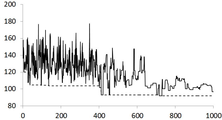
Figure 3.13: Progress of simulated annealing. Solid line shows current solution cost, dashed line best cost so far.
