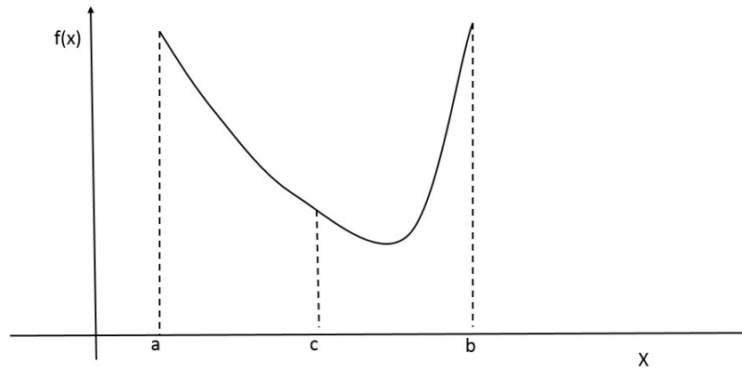
Figure 3.9: Bisection method.
