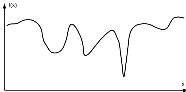
Figure 3.10: Moving downhill from the current location may not lead to the global optimum.
